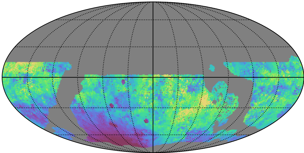
no_long_daily_v3.4_10yrs WFD g band: Median moonDistance
