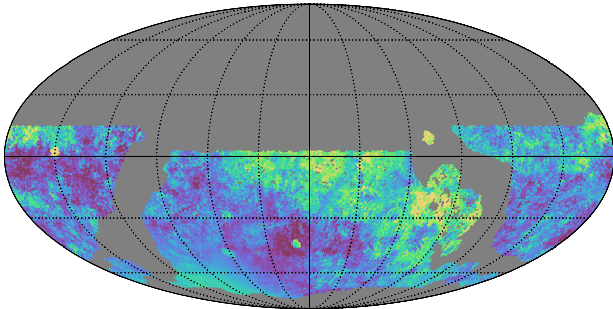
no_long_daily_v3.4_10yrs WFD all bands: Median moonDistance
