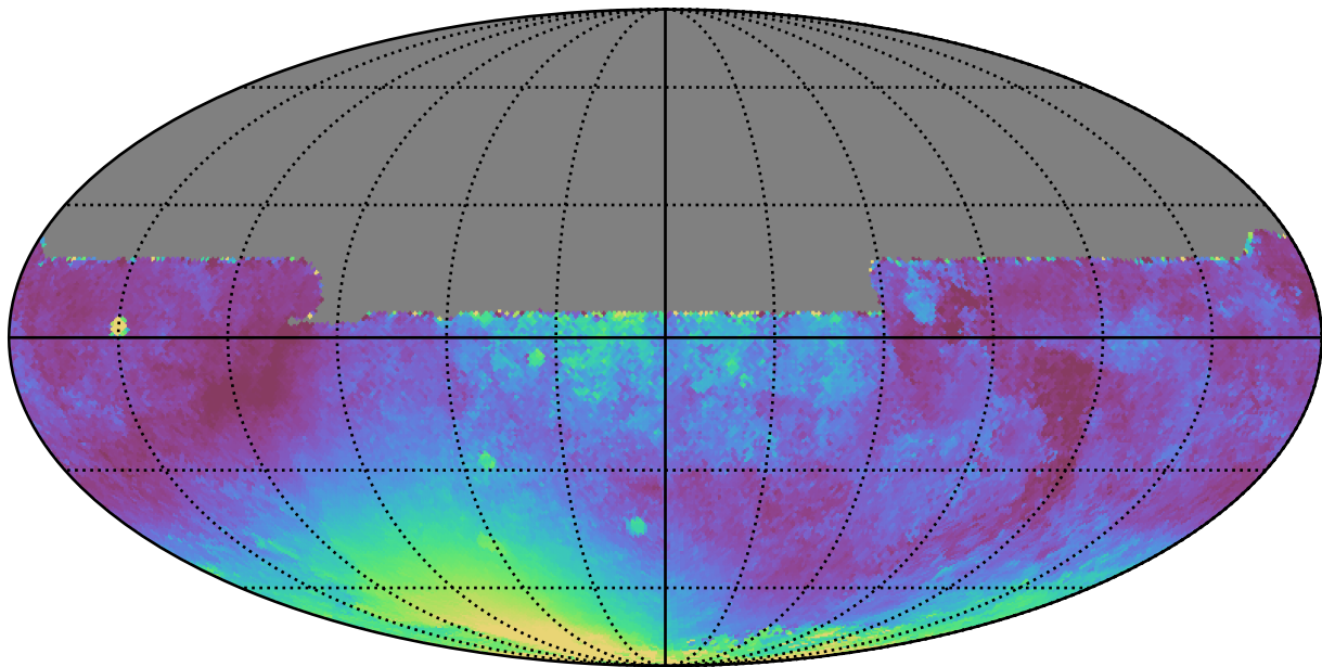
no_long_daily_v3.4_10yrs All sky y band: Median moonDistance
