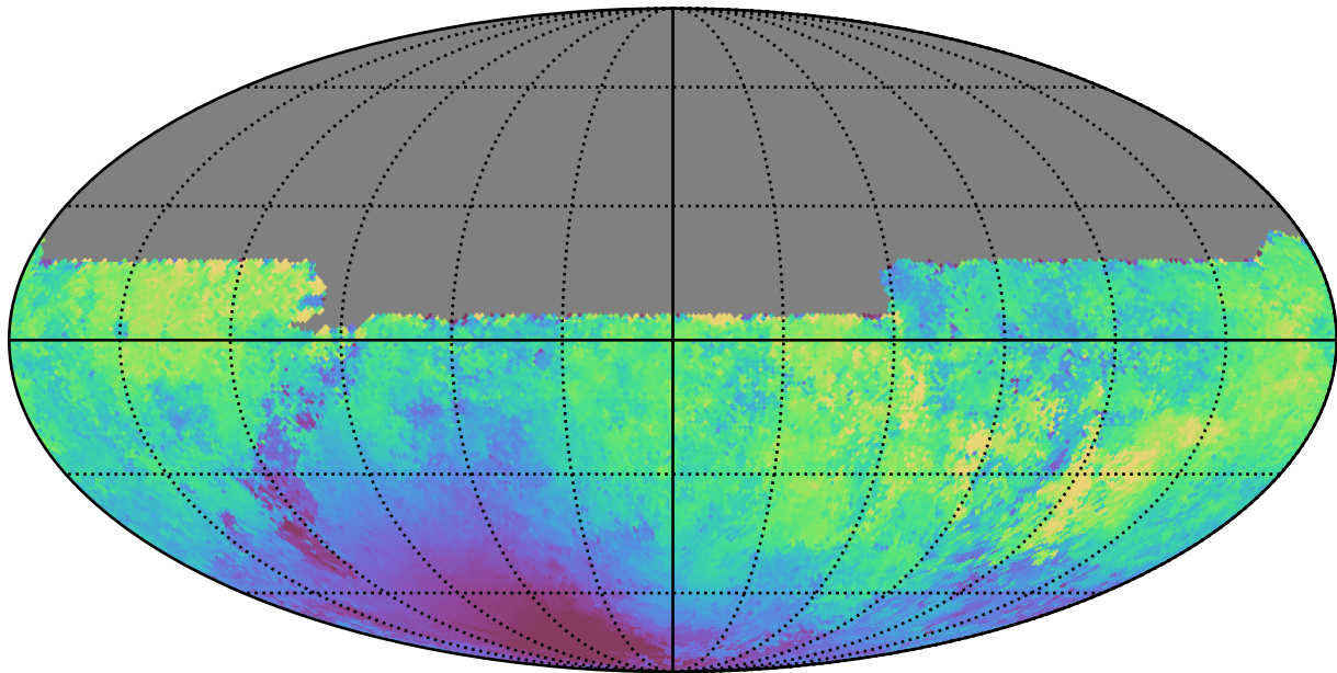
no_long_daily_v3.4_10yrs All sky u band: Median moonDistance
