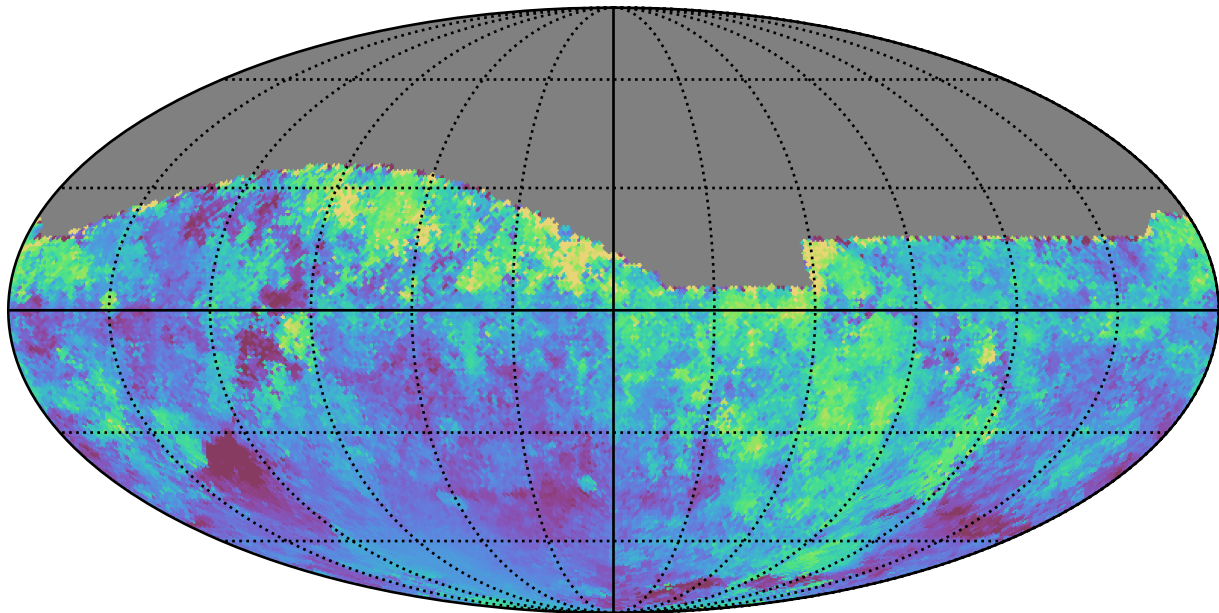
no_long_daily_v3.4_10yrs All sky i band: Median moonDistance
