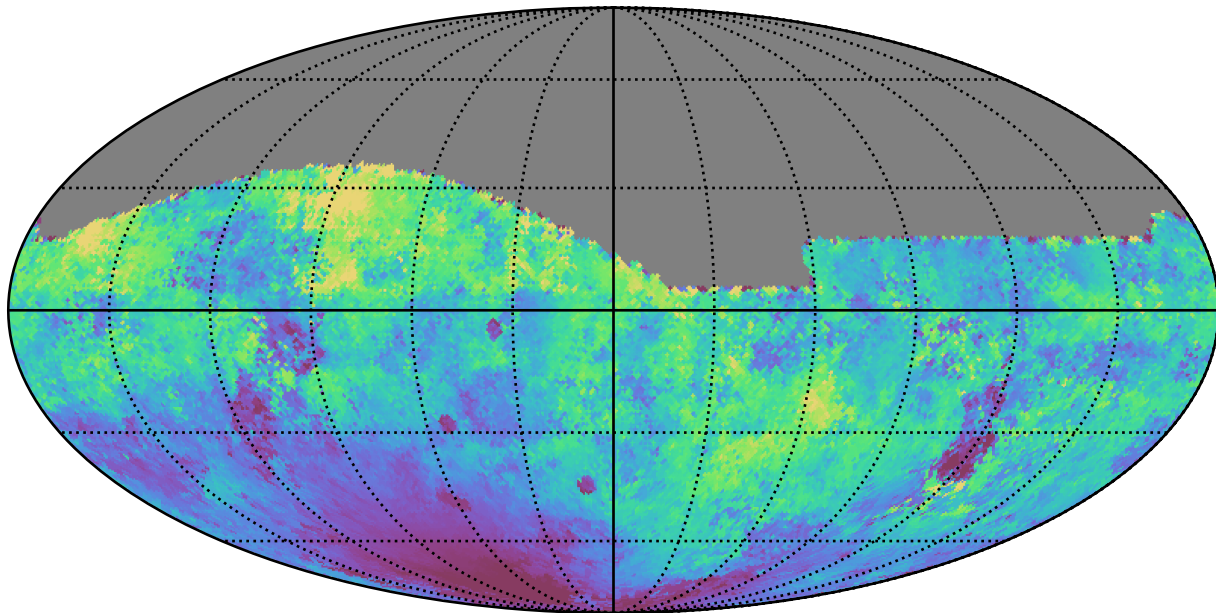
no_long_daily_v3.4_10yrs All sky g band: Median moonDistance
