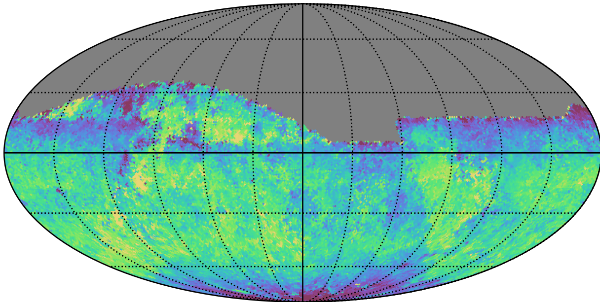
no_long_daily_v3.4_10yrs Yr 1 all bands: Median fiveSigmaDepth
