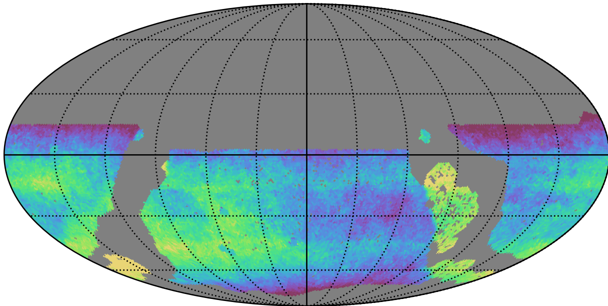
no_long_daily_v3.4_10yrs WFD all bands: Median fiveSigmaDepth
