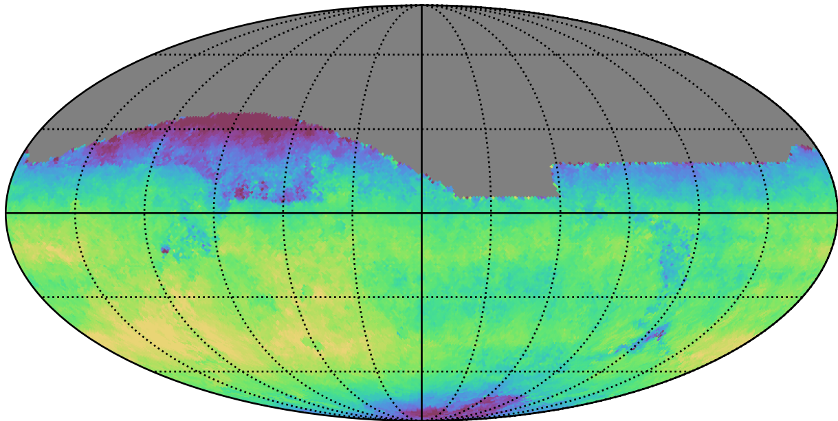
no_long_daily_v3.4_10yrs All sky z band: Median fiveSigmaDepth
