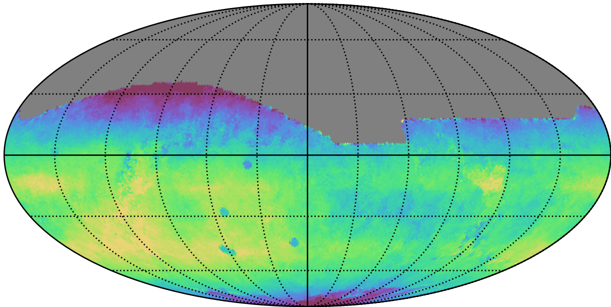
no_long_daily_v3.4_10yrs All sky r band: Median fiveSigmaDepth
