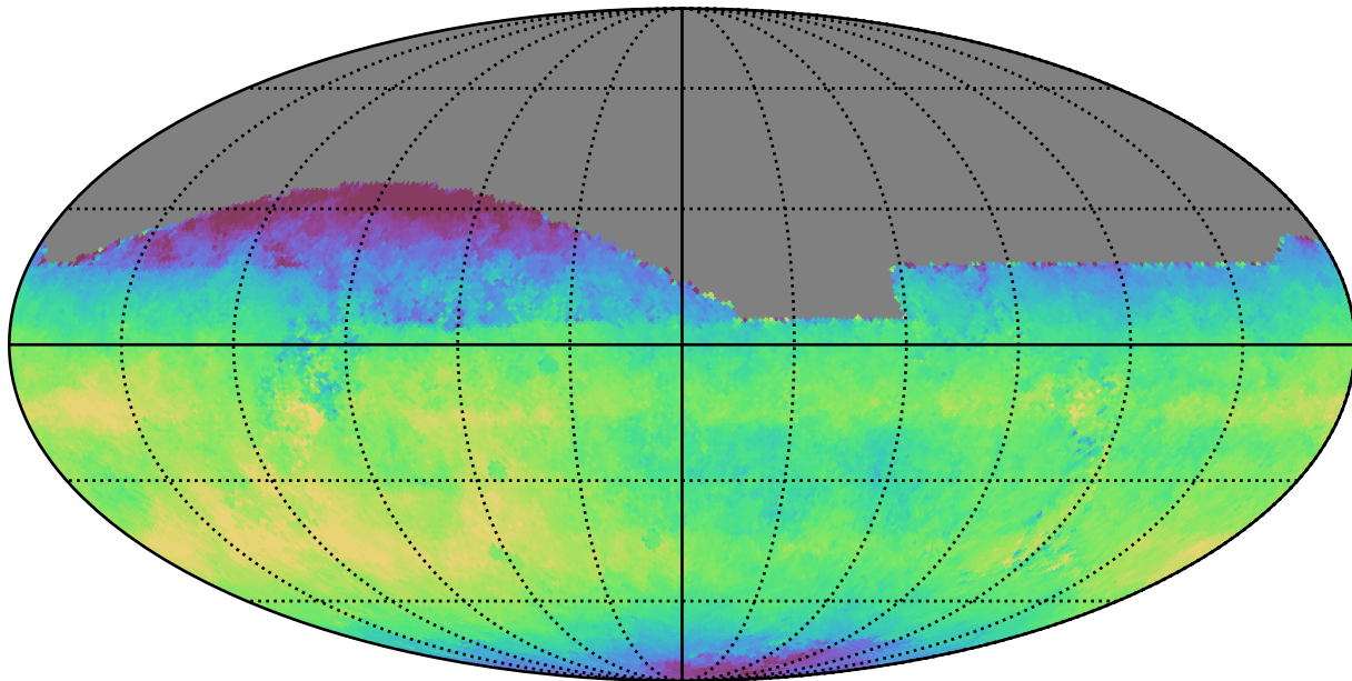
no_long_daily_v3.4_10yrs All sky i band: Median fiveSigmaDepth
