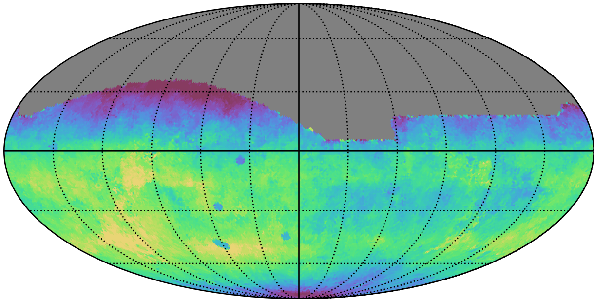
no_long_daily_v3.4_10yrs All sky g band: Median fiveSigmaDepth
