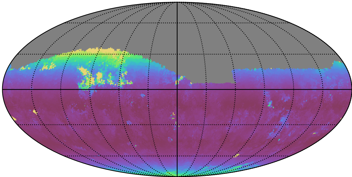
no_long_daily_v3.4_10yrs Yr 1 z band: Median airmass
