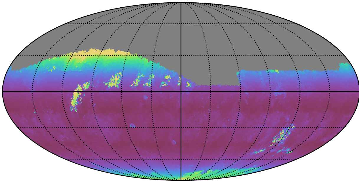
no_long_daily_v3.4_10yrs Yr 1 r band: Median airmass
