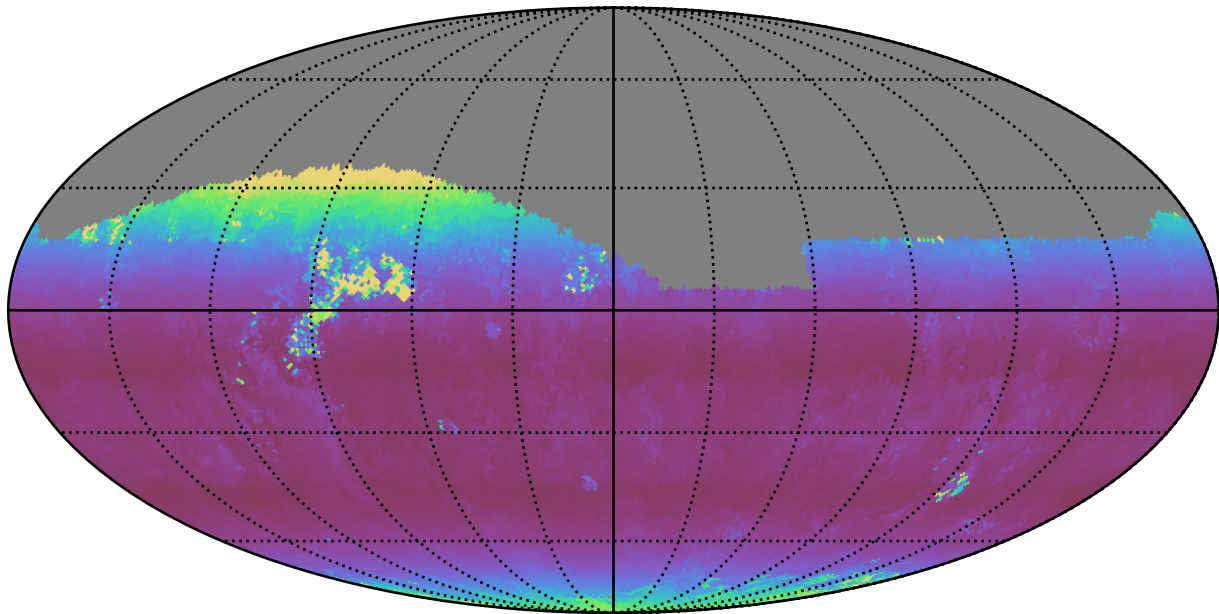
no_long_daily_v3.4_10yrs Yr 1 i band: Median airmass
