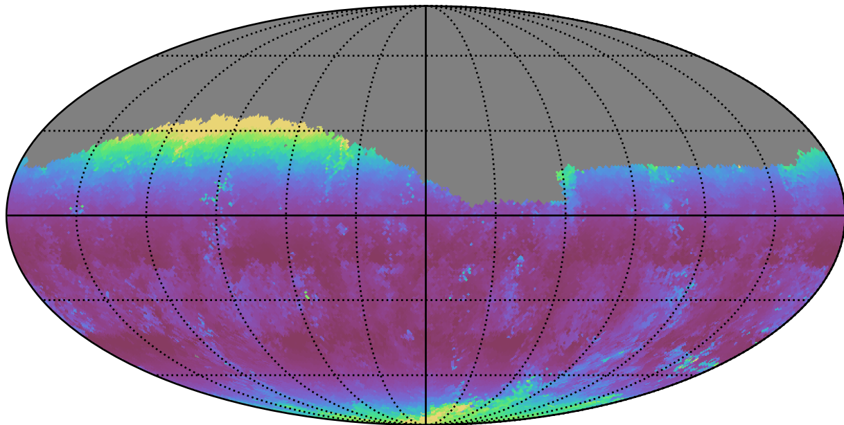
no_long_daily_v3.4_10yrs Yr 1 g band: Median airmass
