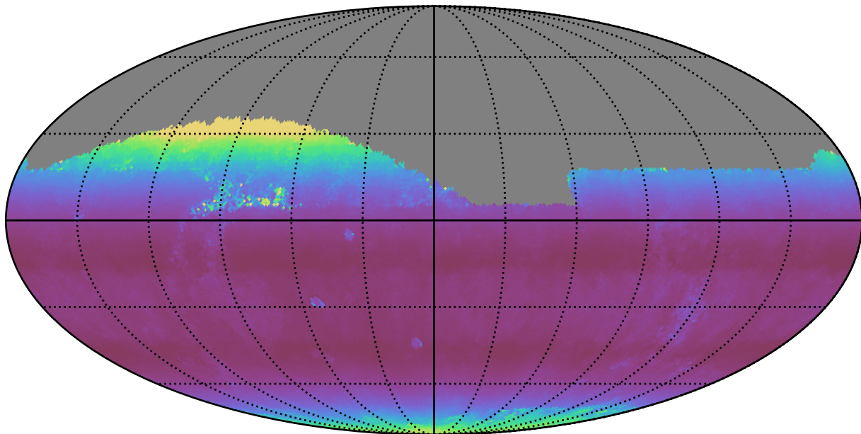
no_long_daily_v3.4_10yrs Yr 1 all bands: Median airmass
