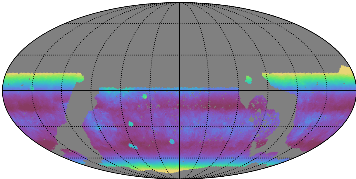
no_long_daily_v3.4_10yrs WFD z band: Median airmass
