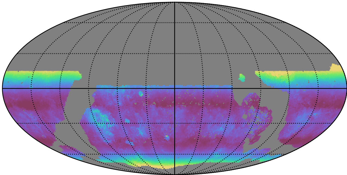
no_long_daily_v3.4_10yrs WFD u band: Median airmass
