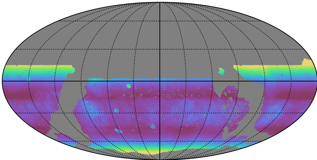
no_long_daily_v3.4_10yrs WFD r band: Median airmass
