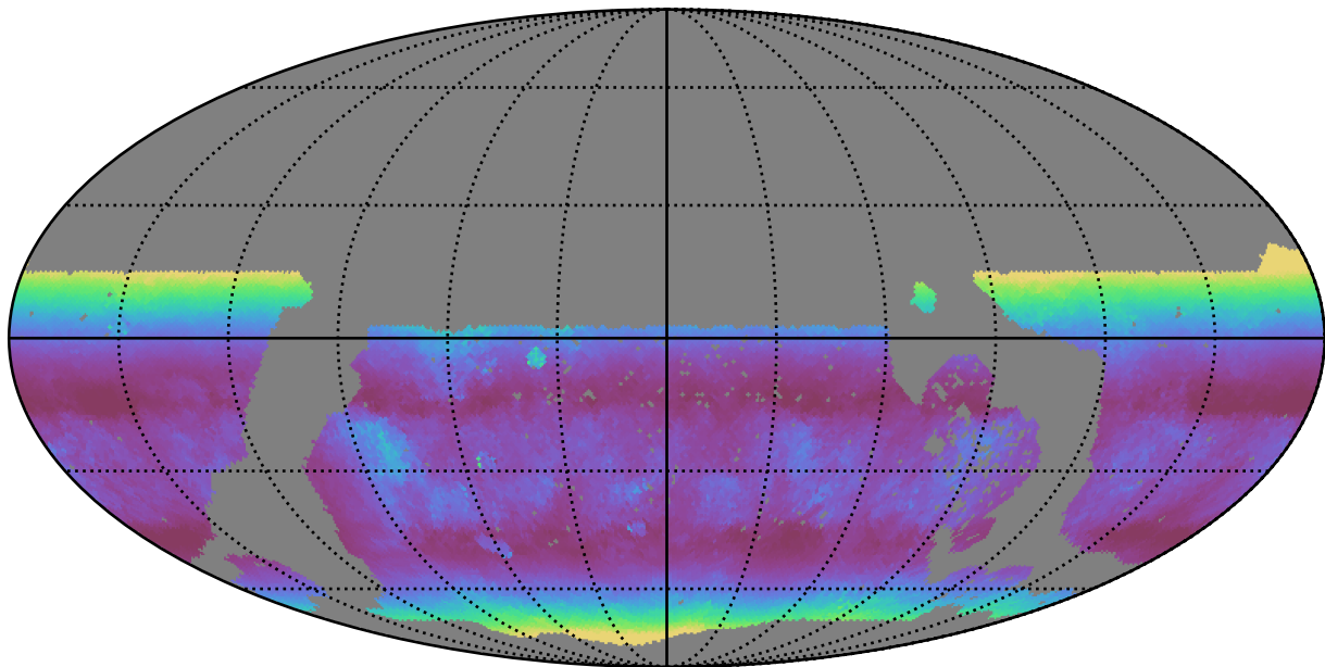
no_long_daily_v3.4_10yrs WFD g band: Median airmass
