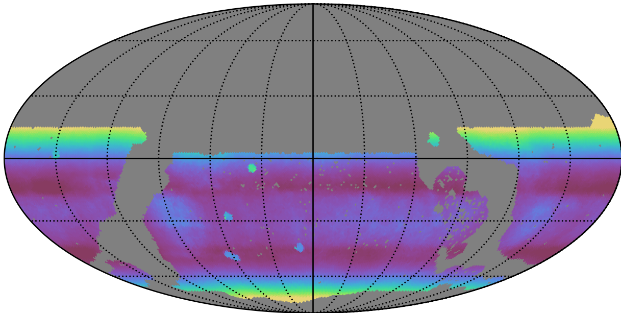
no_long_daily_v3.4_10yrs WFD all bands: Median airmass
