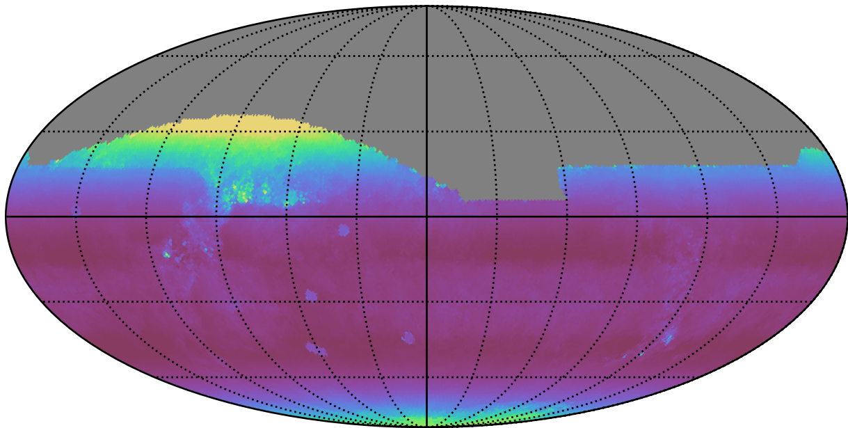
no_long_daily_v3.4_10yrs All sky z band: Median airmass
