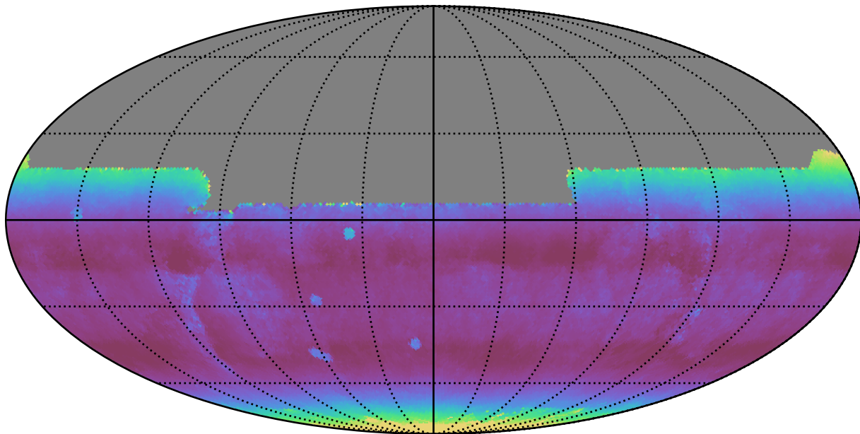
no_long_daily_v3.4_10yrs All sky y band: Median airmass
