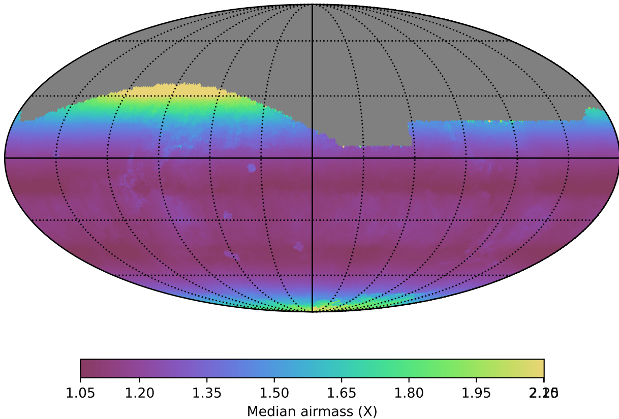
no_long_daily_v3.4_10yrs All sky r band: Median airmass
