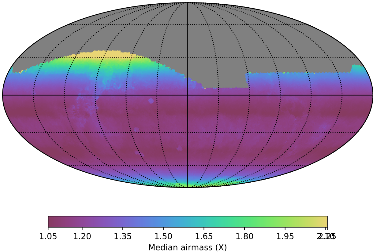
no_long_daily_v3.4_10yrs All sky i band: Median airmass
