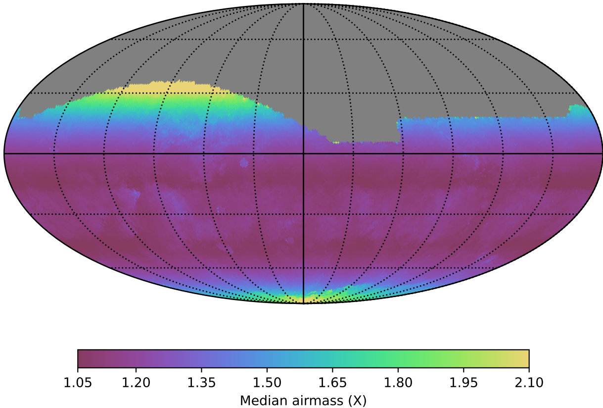
no_long_daily_v3.4_10yrs All sky g band: Median airmass
