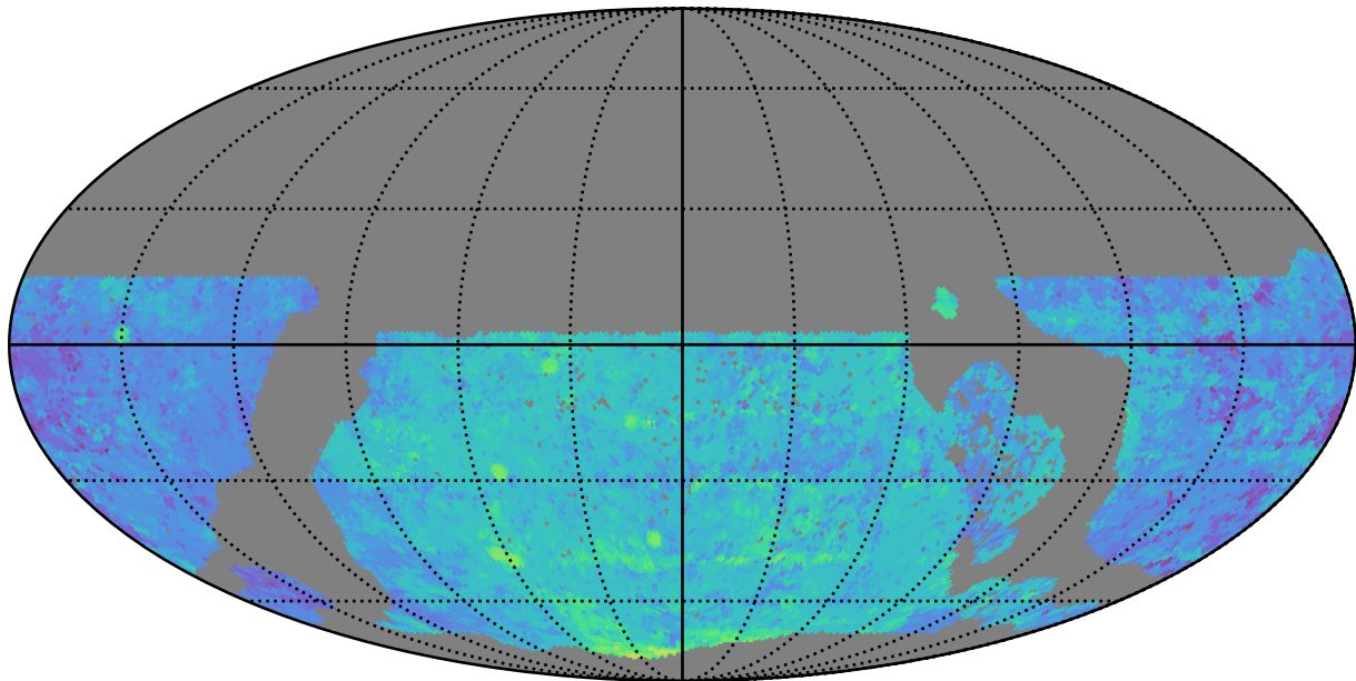
no_long_daily_v3.4_10yrs WFD y band: Median Season Length
