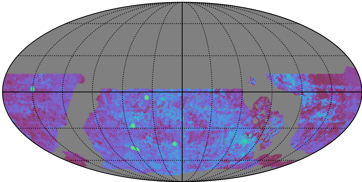
no_long_daily_v3.4_10yrs WFD u band: Median Season Length
