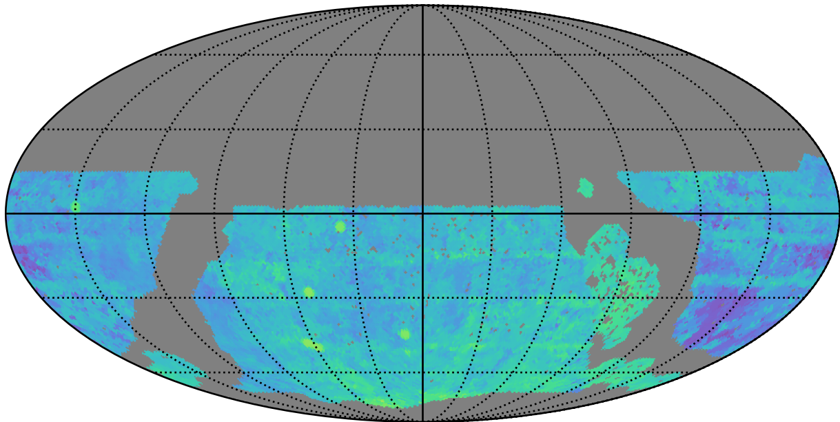
no_long_daily_v3.4_10yrs WFD r band: Median Season Length
