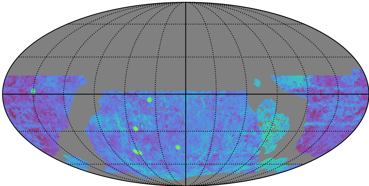
no_long_daily_v3.4_10yrs WFD g band: Median Season Length
