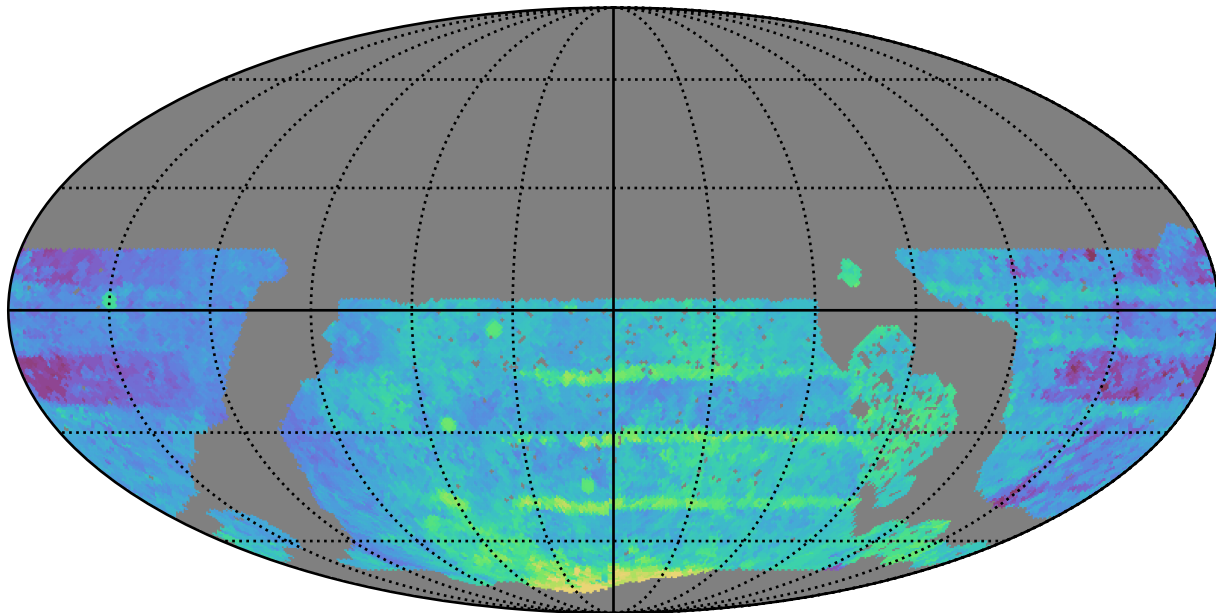
no_long_daily_v3.4_10yrs WFD all bands: Median Season Length
