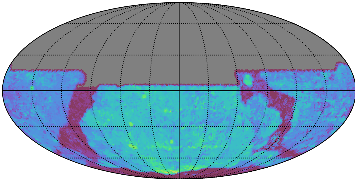
no_long_daily_v3.4_10yrs All sky y band: Median Season Length
