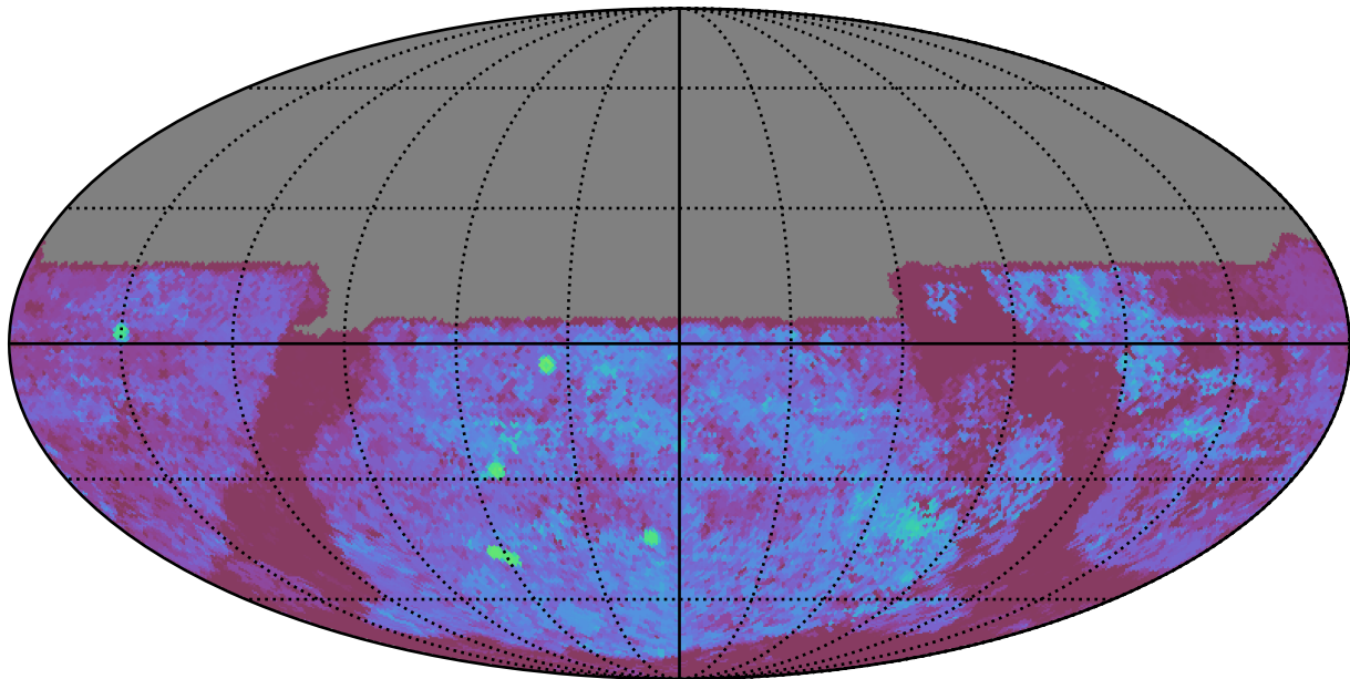
no_long_daily_v3.4_10yrs All sky u band: Median Season Length
