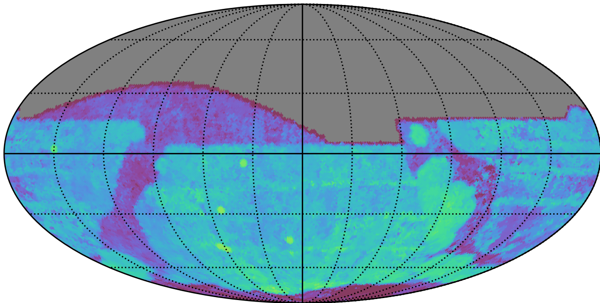
no_long_daily_v3.4_10yrs All sky r band: Median Season Length
