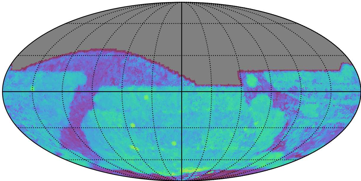
no_long_daily_v3.4_10yrs All sky i band: Median Season Length
