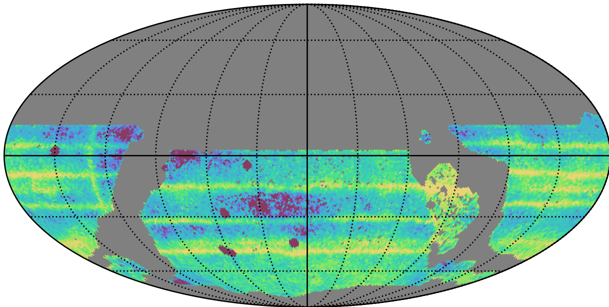
no_long_daily_v3.4_10yrs WFD: Median Intra-Night Gap
