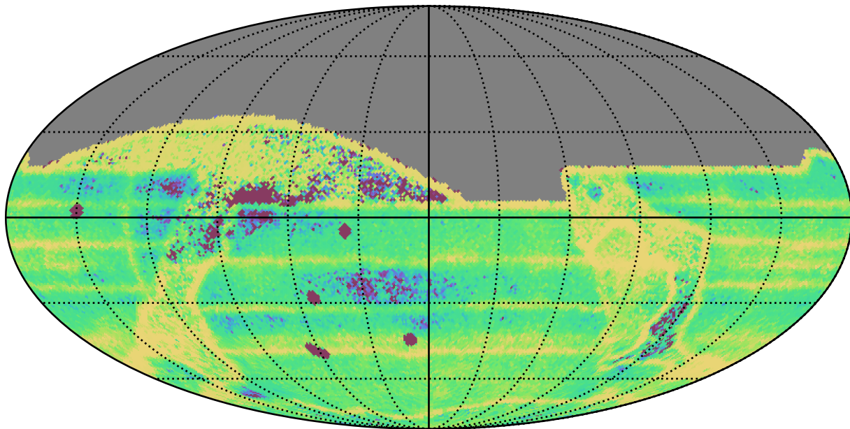
no_long_daily_v3.4_10yrs All sky: Median Intra-Night Gap
