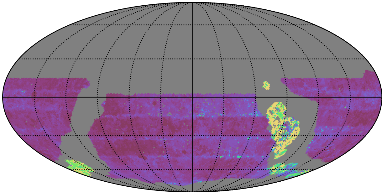
no_long_daily_v3.4_10yrs WFD u band: Median Inter-Night Gap
