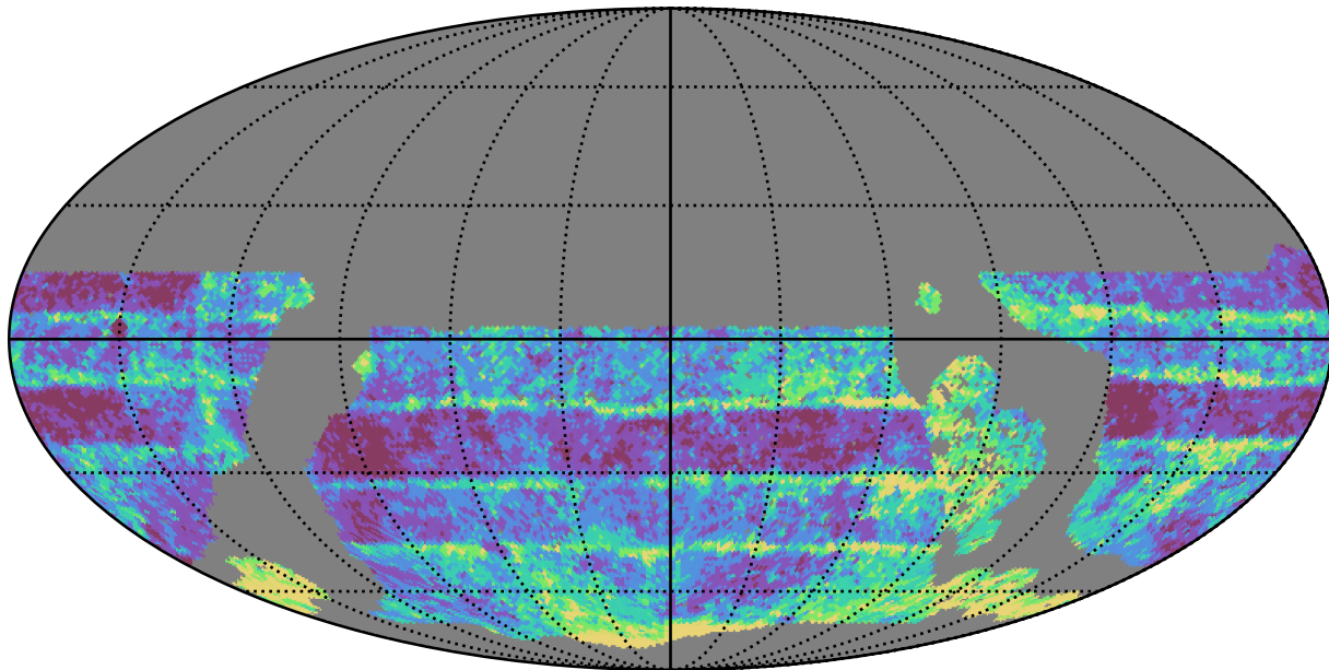
no_long_daily_v3.4_10yrs WFD r band: Median Inter-Night Gap
