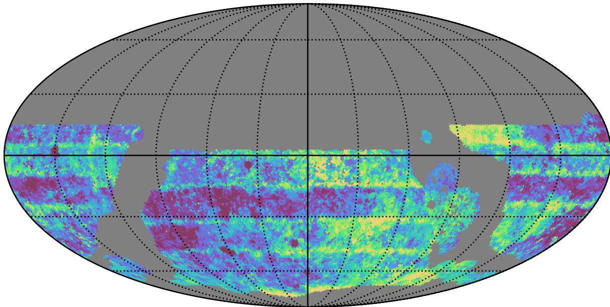
no_long_daily_v3.4_10yrs WFD g band: Median Inter-Night Gap
