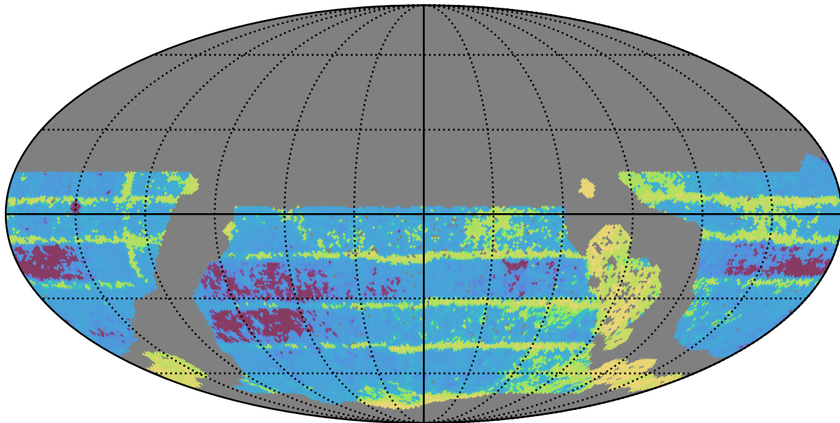
no_long_daily_v3.4_10yrs WFD all bands: Median Inter-Night Gap
