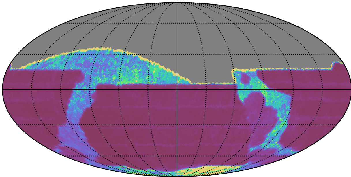
no_long_daily_v3.4_10yrs All sky z band: Median Inter-Night Gap
