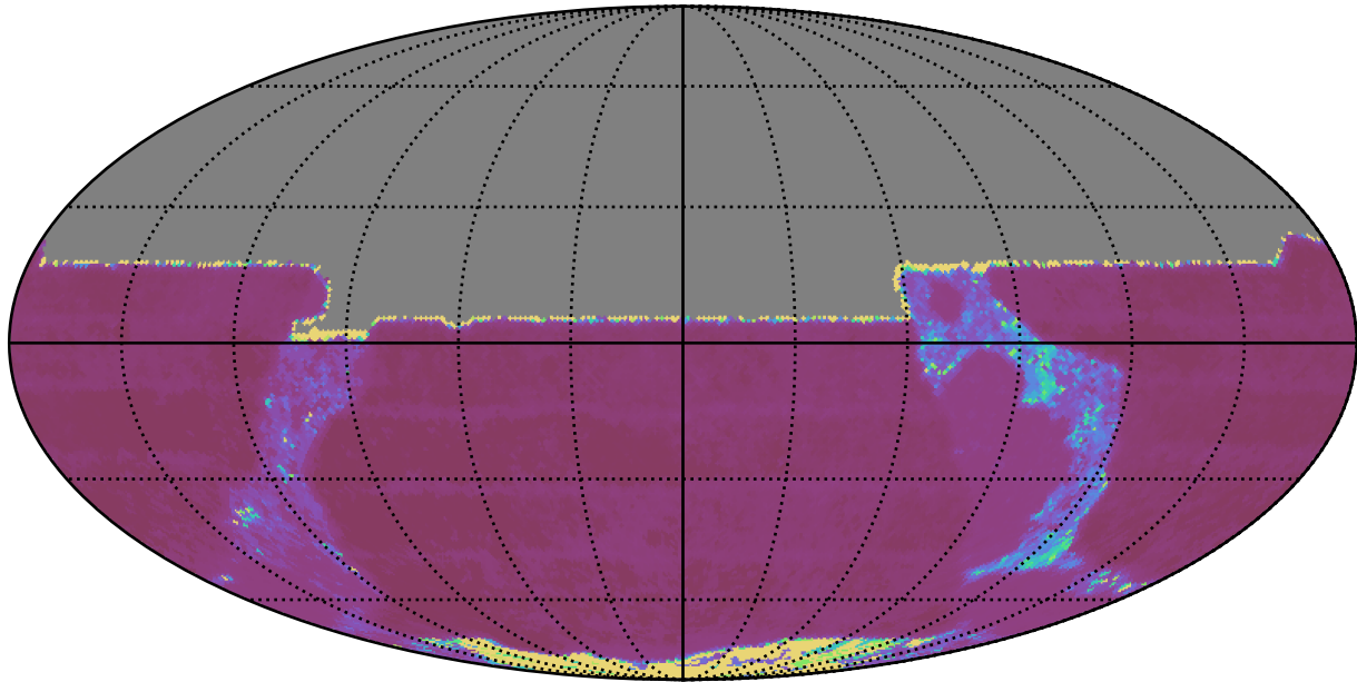
no_long_daily_v3.4_10yrs All sky y band: Median Inter-Night Gap
