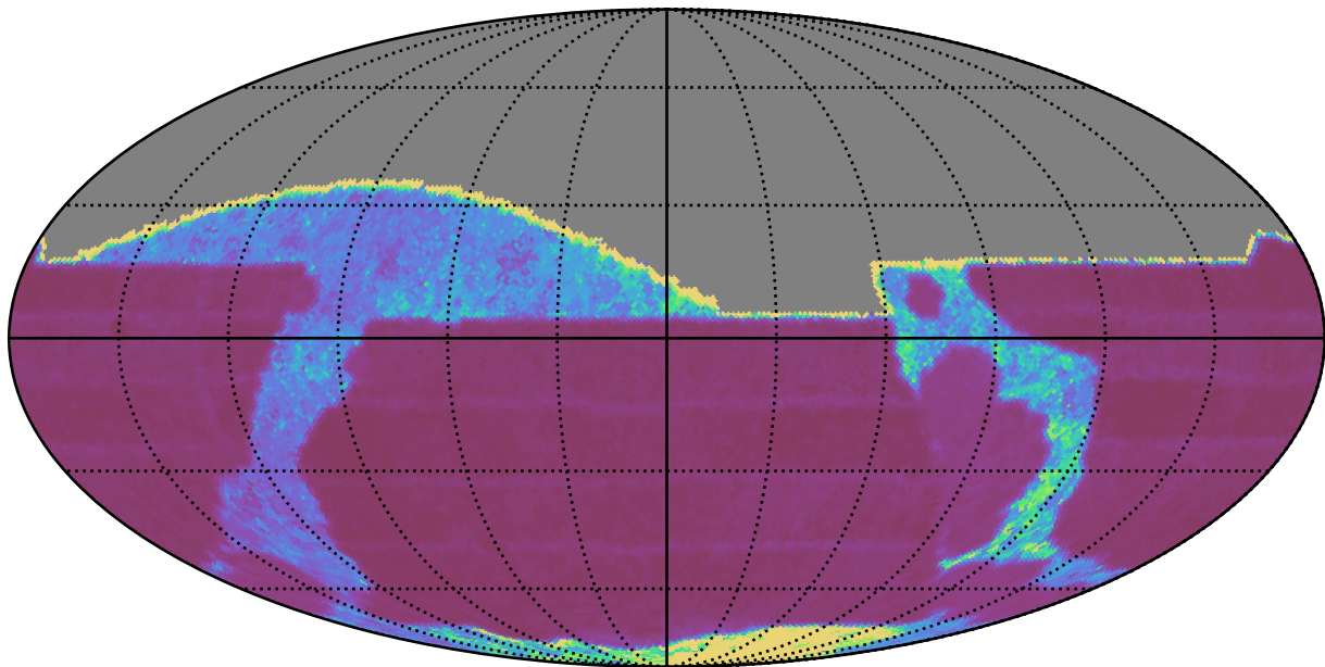
no_long_daily_v3.4_10yrs All sky i band: Median Inter-Night Gap
