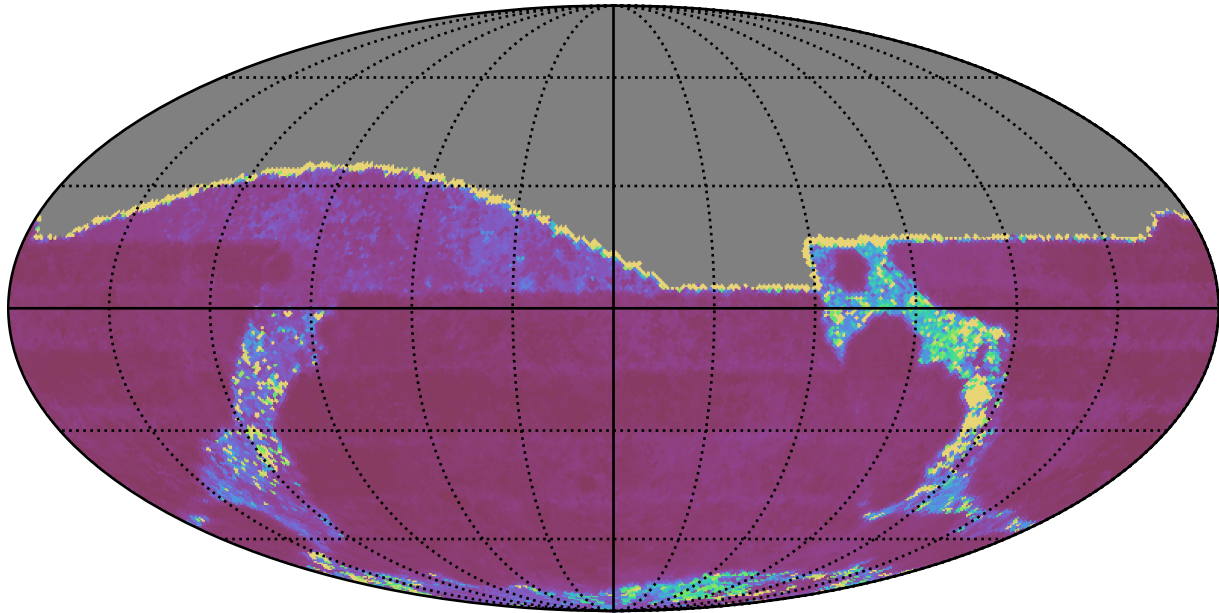
no_long_daily_v3.4_10yrs All sky g band: Median Inter-Night Gap
