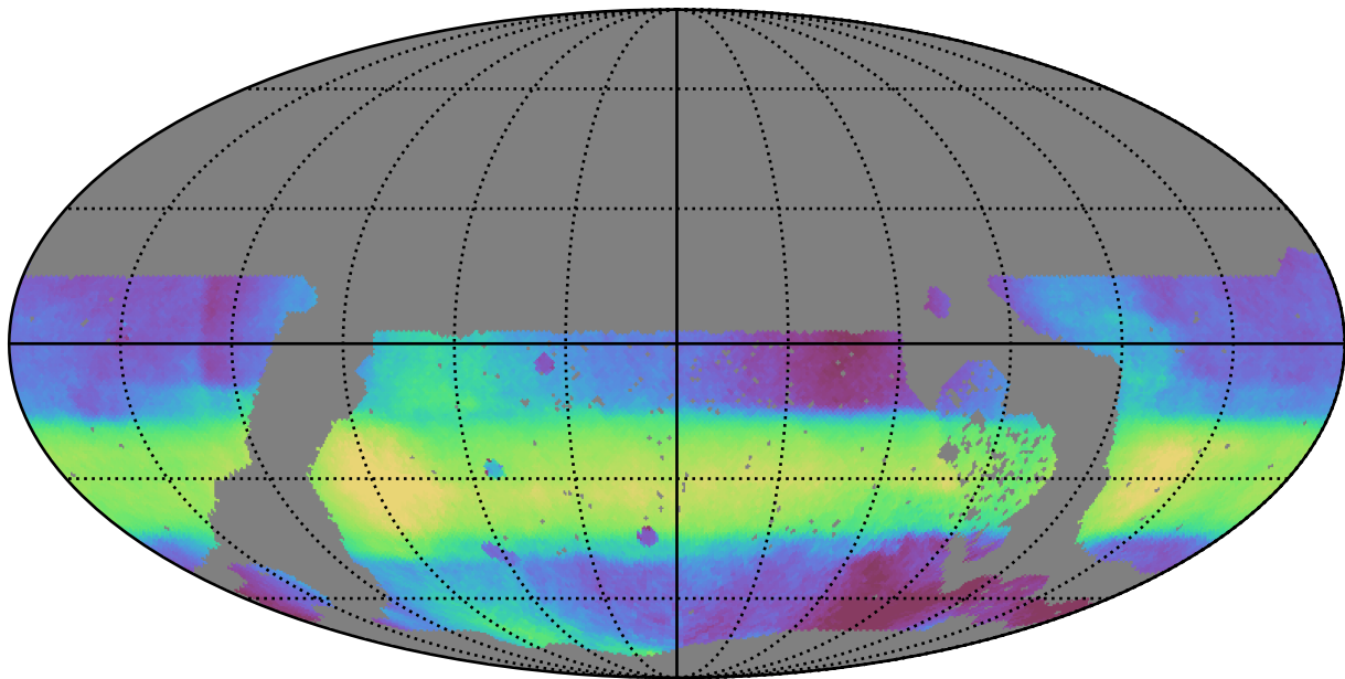
no_long_daily_v3.4_10yrs WFD all bands: Median HA
