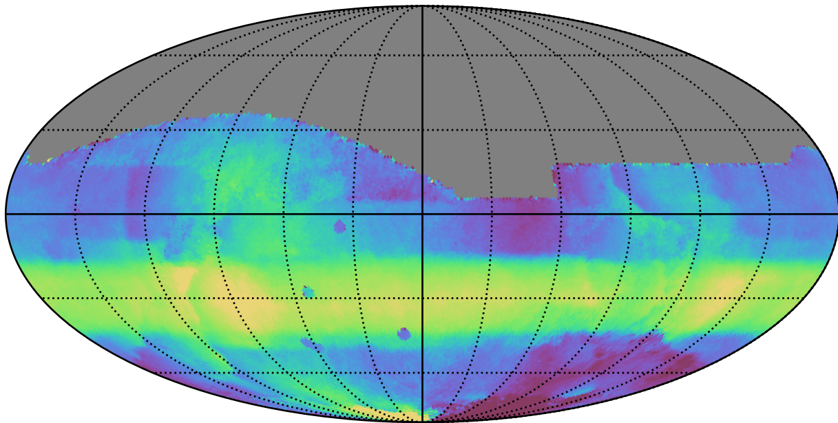
no_long_daily_v3.4_10yrs All sky all bands: Median HA
