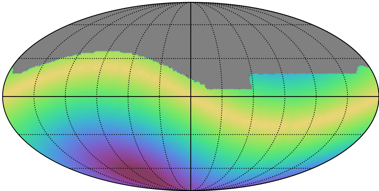
no_long_daily_v3.4_10yrs All sky all bands: Max solarElong
