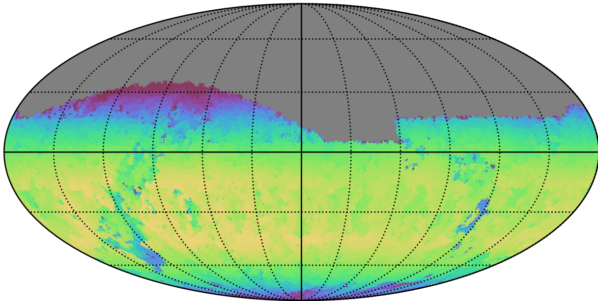
no_long_daily_v3.4_10yrs Yr 1 z band: Max skyBrightness
